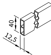
stand-off strip for wall sealing profile
